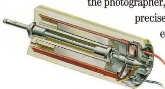
CORELESS MOTOR
